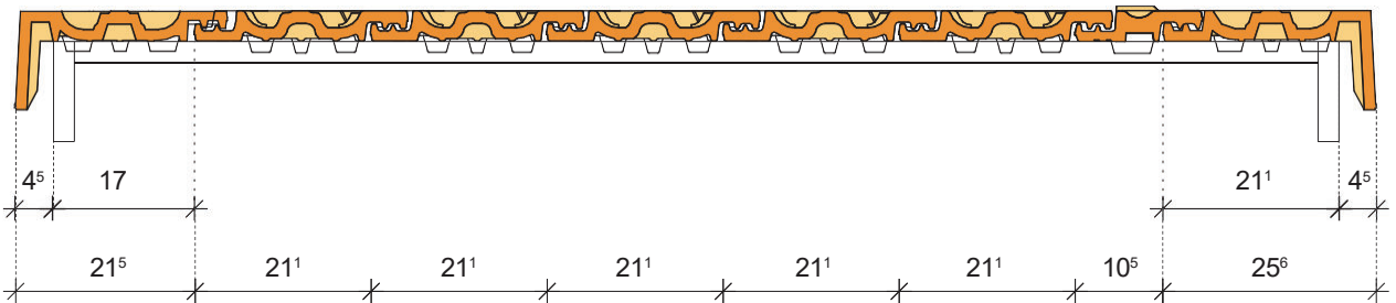
Ortgangziegel links
